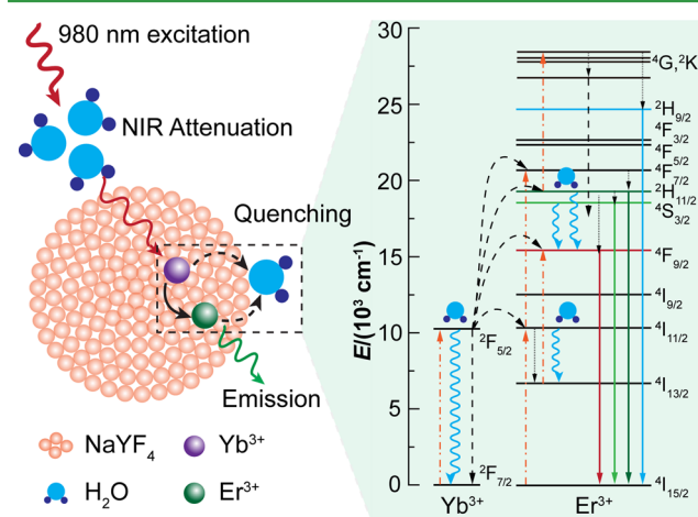
Figure 1. Schematic illustration of water molecule induced upconversion emission quenching of NaYF 4 :Yb/Er nanoparticles. Water molecules can absorb part of the excitation energy before excitation light reaches nanoparticles. Upon excitation of the nanoparticle, Yb 3+ and Er 3+ ions, in their excitation states, can transfer their energy to the nearby water molecules. Consequently, the upconversion emission is suppressed. Energy level diagrams on the right panel illustrate the proposed upconversion mechanisms. The dashed-dotted, dashed, dotted, wavy, and solid arrows represent photon excitation, energy transfer, multiphonon relaxation, water induced energy depletion, and emission process, respectively.
