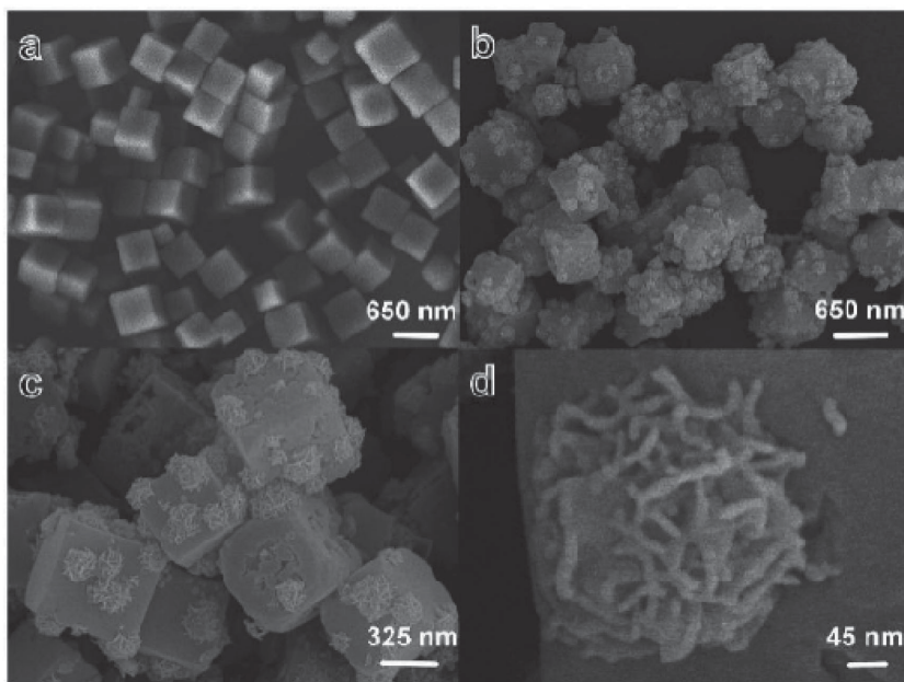
Figure 1. SEM images of a) MHCF and b–d) MnO x –MHCF at different magnifications.
